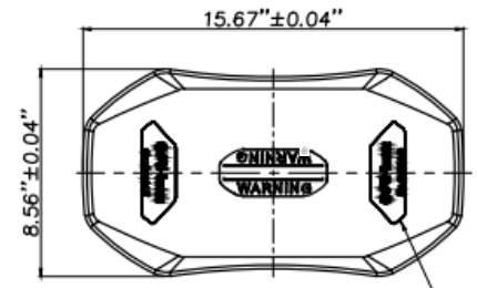
STUD MOUNT WITH 3-WIRE CABLE
