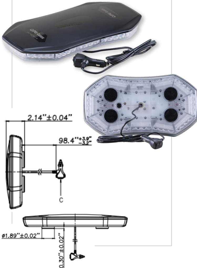
MAGNET MOUNT WITH CIGARETTE LIGHTER CONNECTOR
