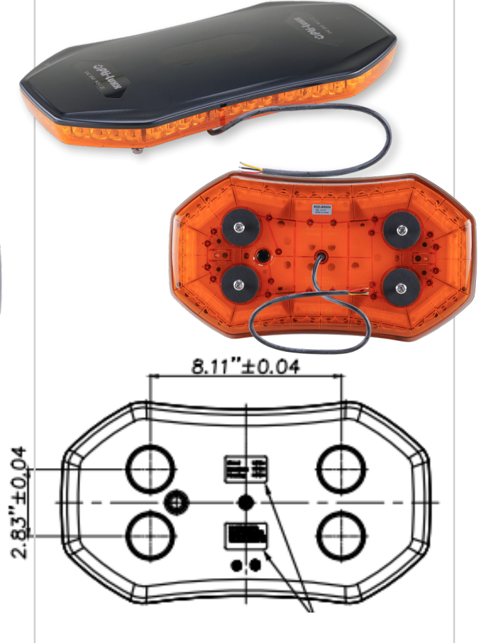
STUD MOUNT WITH 3-WIRE CABLE
